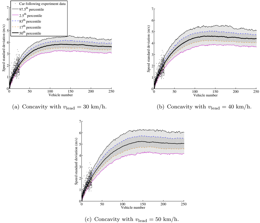
Figure 6. Concavity revealed in car-following platoon simulations when the leading vehicle in the platoon drives at (a) v_{\text{lead}} = 30 km/h, (b) v_{\text{lead}} = 40 km/h and (c) v_{\text{lead}} = 50 km/h. We used \beta = 0.06 and \sigma = 0.055 . The shaded areas illustrate the 95%-percentage (between 97.5 th and 2.5 th percentile) and 66%-percentage (between 83 th and 17 th percentile) of the 500 simulations. The bold curve is the mean value of the simulation results. The dots in Figure 6 are the speed standard deviation obtained from Jiang's car-following experiments.
