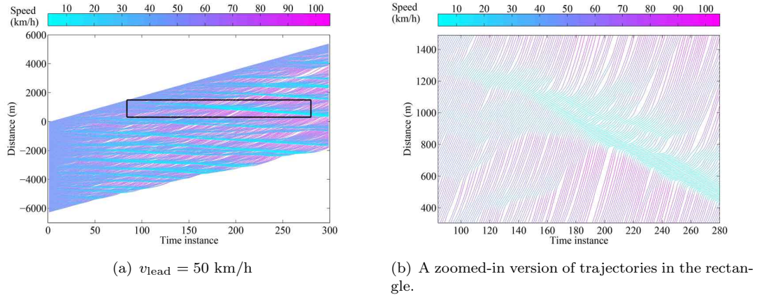
Figure 5. Samples of vehicular trajectories in simulations. The color map indicates the vehicular speed. v_{\text{lead}} = 50 km/h in this sample. An overview of the simulation results are given in (a). The trajectories in the rectangle in (a) is shown in (b) for a better visualization. In simulations, \beta = 0.06 and \sigma = 0.06 .
